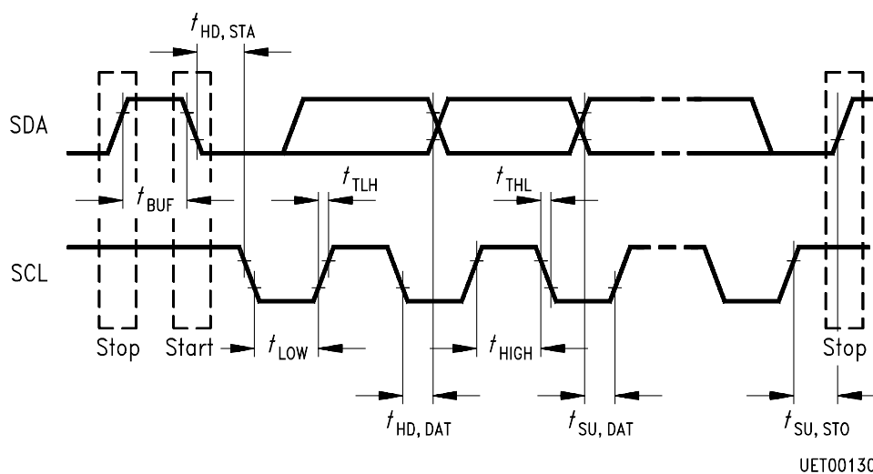
Figure 3 I²C-Bus Timing
