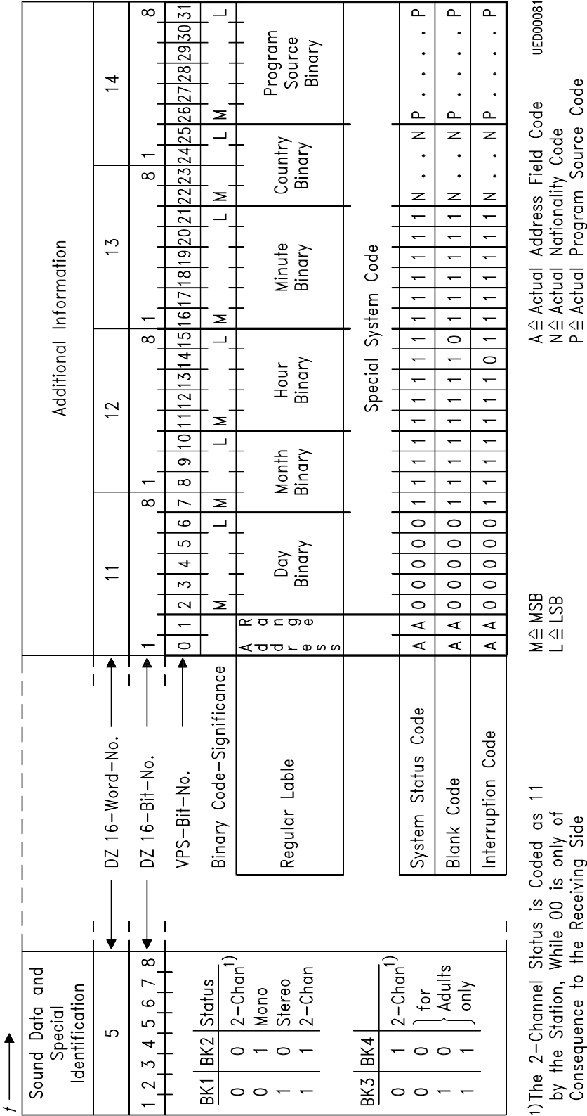
Figure 7 Data Format of Additional Information in Data Line 16
