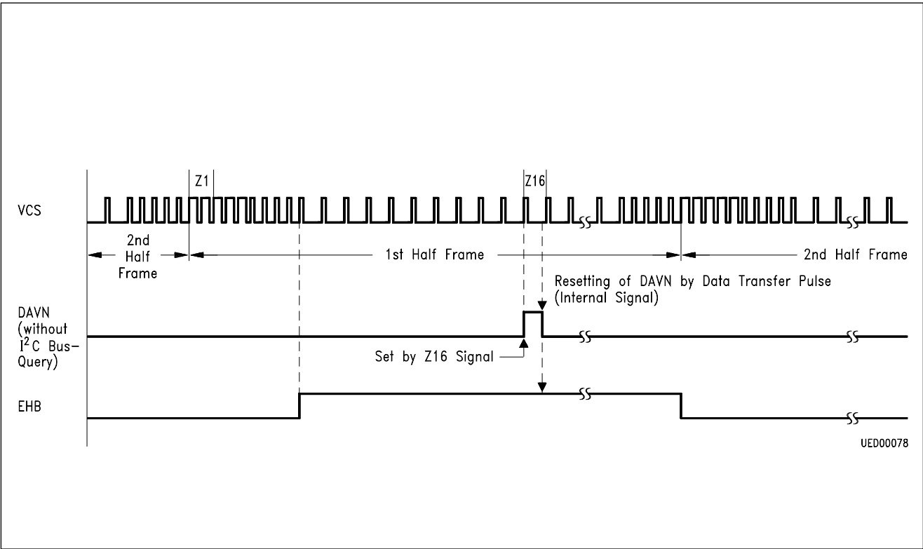
Figure 4 VCS-DAVN-EHB Signal
