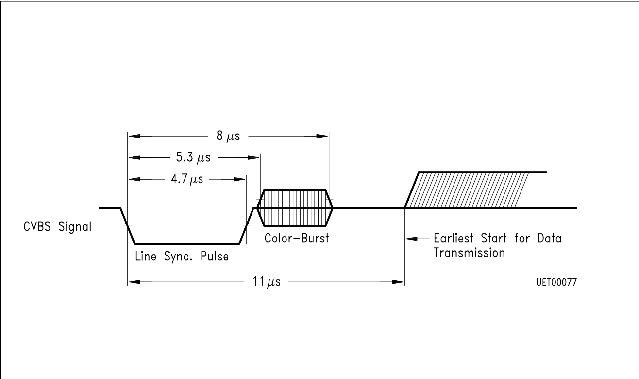
Figure 3 Video Signal
