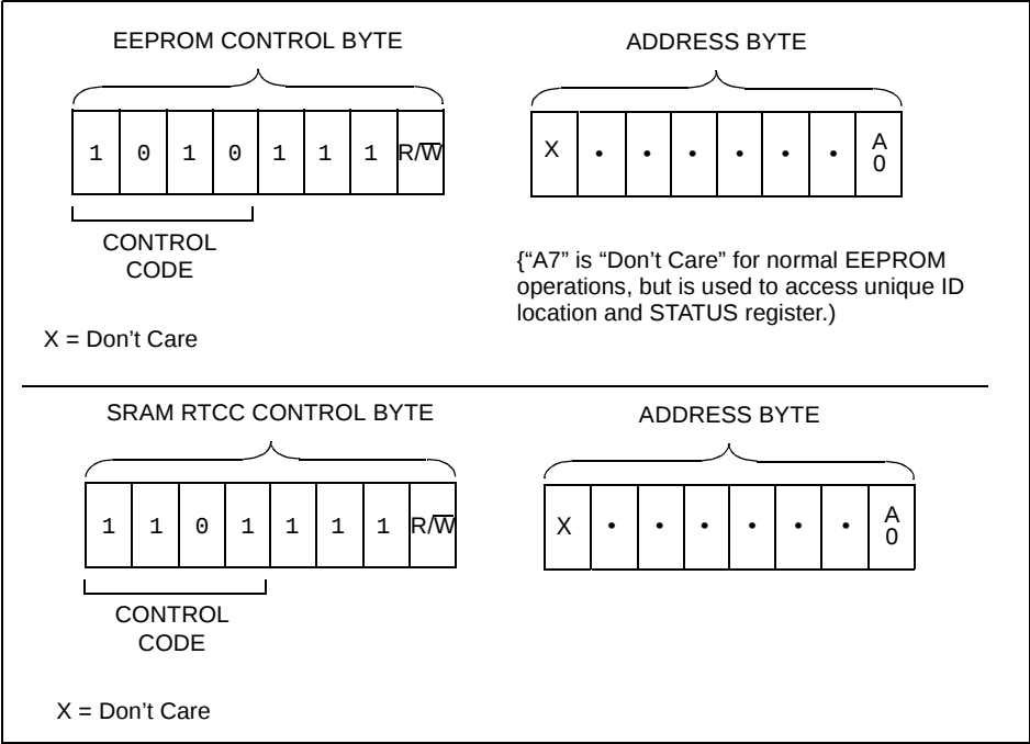
FIGURE 3-3: ADDRESS SEQUENCE BIT ASSIGNMENTS
