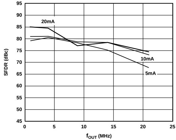
Figure 10. SFDR vs. f_{OUT} and I_{OUTS} at 65 MSPS and 0 dBFS
