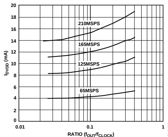
Figure 32. I_{DVDD} vs. Ratio at DVDD = 3.3 V
