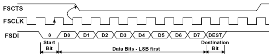
Figure 4-2 Fast Opto-Isolated Serial Interface Input Data Format
