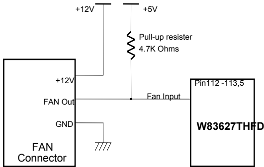
Figure 5-4. Fan with Tach Pull-Up to +5V
