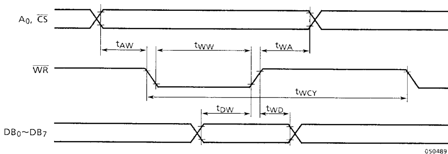
Figure 12.2 WRITE TIMING
