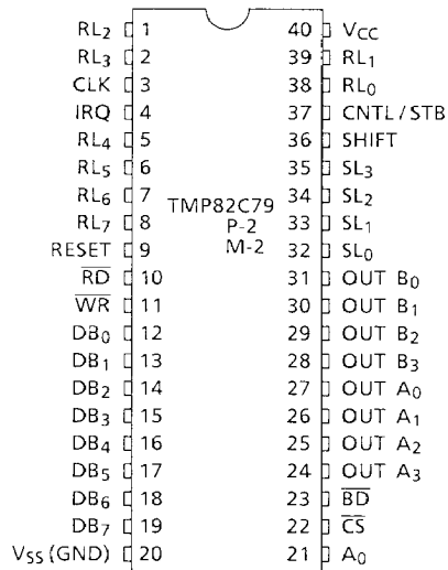
Figure 3.1 Pin Connection
