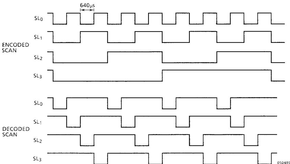
figure 12.4 scan timing
