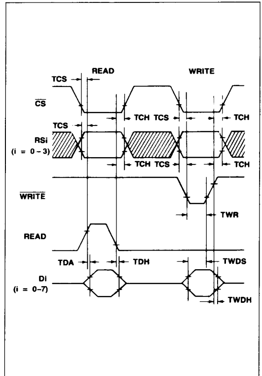
Microprocessor Interface Timing Waveforms
