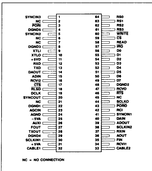
R48MF X Pin Assignments
