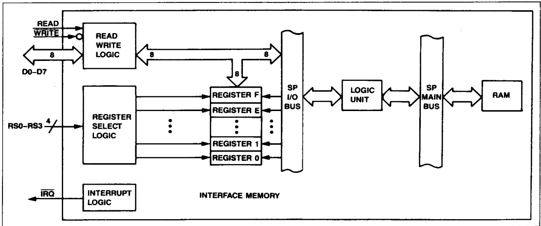
R48MFX Host Processor Interface
