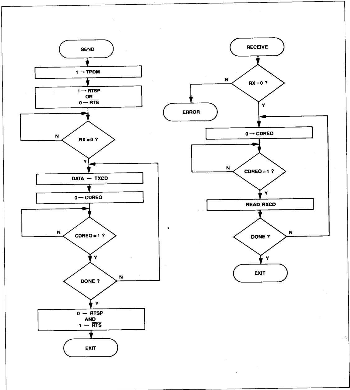
Channel Data Parallel Mode Control
