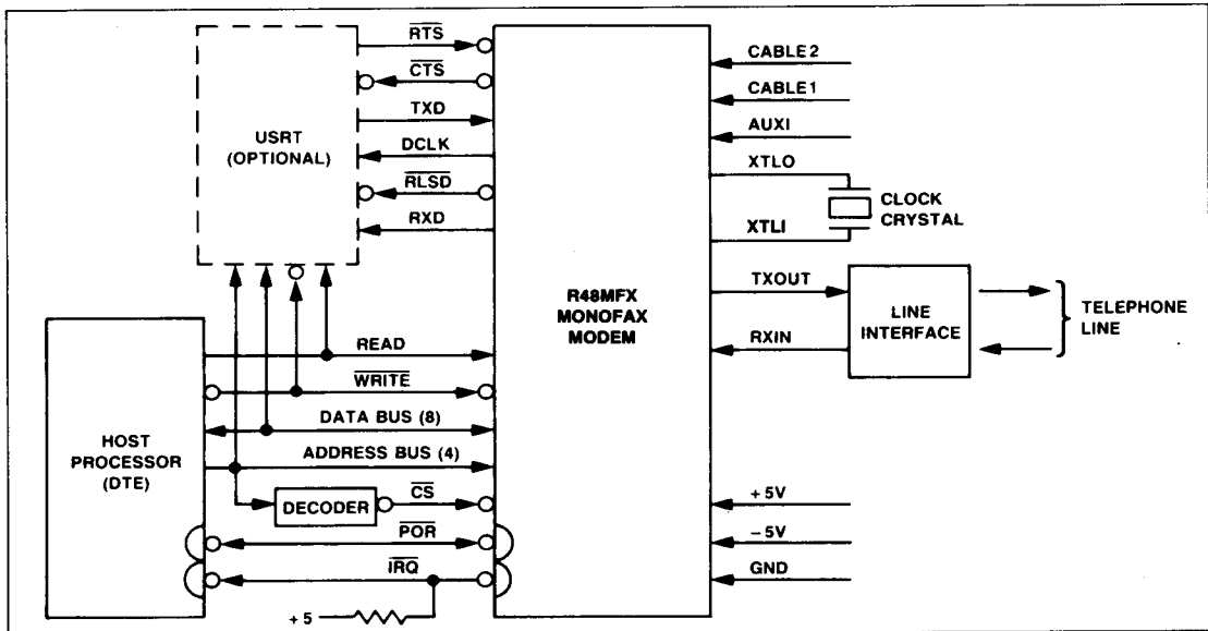
R48MFX Functional Interconnect Diagram
