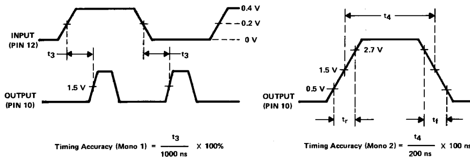
VOLTAGE WAVEFORMS
