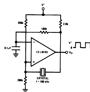
Figure 22. Crystal Controlled Oscillator
