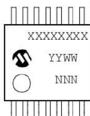
14-Lead TSSOP (4.4mm) (MCP604 Only)
