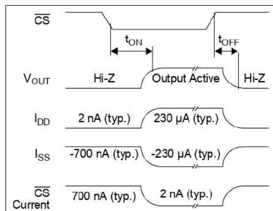
FIGURE 1-1: MCP603 Chip Select ( \overline{\text{CS}} ) Timing Diagram.
