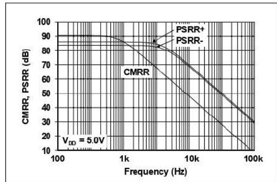
FIGURE 2-16: CMRR, PSRR vs. Frequency.
