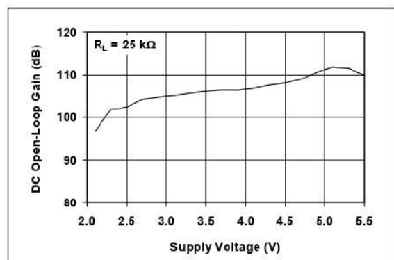
FIGURE 2-18: DC Open-Loop Gain vs. Supply Voltage.
