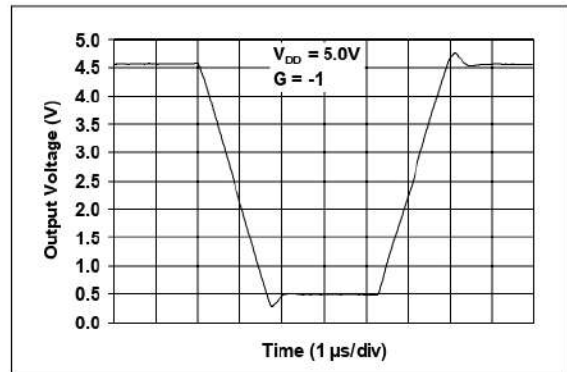
FIGURE 2-28: Large Signal Inverting Pulse Response.
