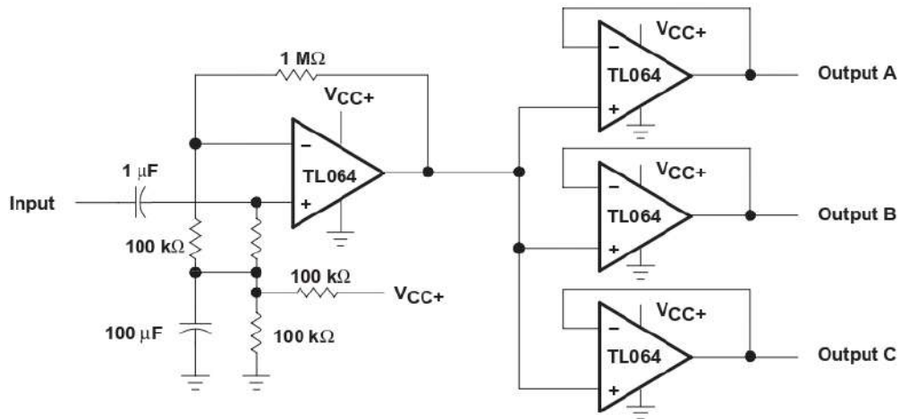
Figure 22. Audio-Distribution Amplifier
