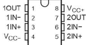
TL062 . . . D, JG, P, PS, OR PW PACKAGE TL062A . . . D, P, OR PS PACKAGE TL062B . . . D OR P PACKAGE (TOP VIEW)
