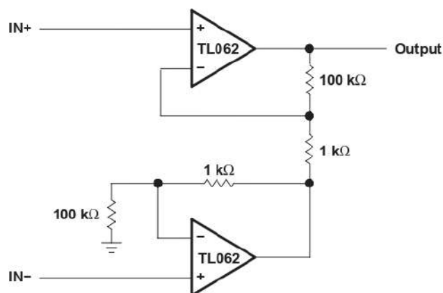
Figure 26. Instrumentation Amplifier
