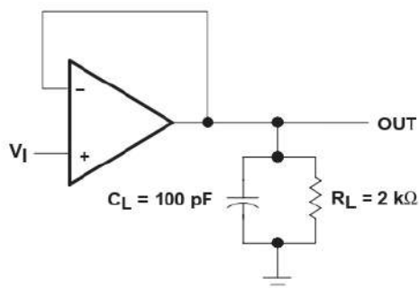
Figure 1. Unity-Gain Amplifier
