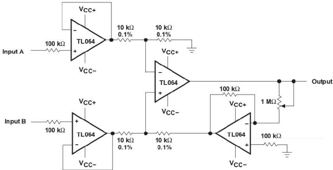
Figure 19. Instrumentation Amplifier
