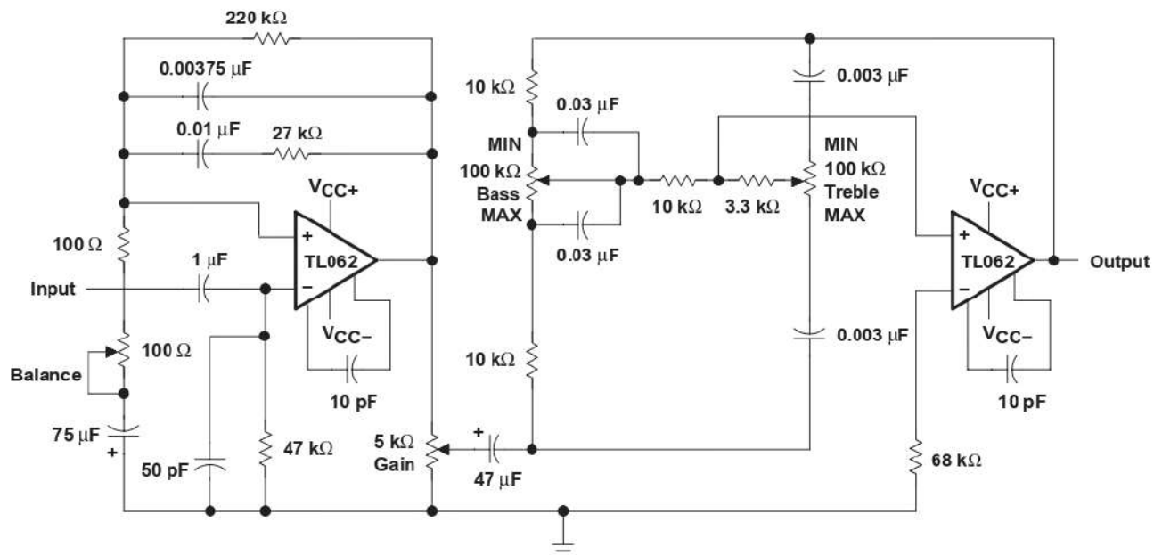
Figure 27. IC Preamplifier
