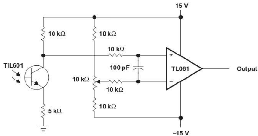
Figure 23. Low-Level Light Detector Preamplifier
