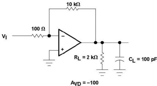
Figure 2. Inverting Amplifier
