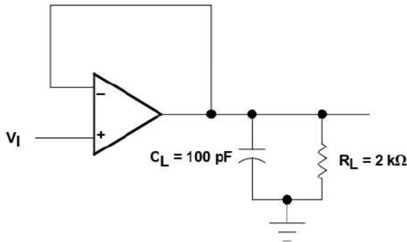
Figure 1. Unity-Gain Amplifier
