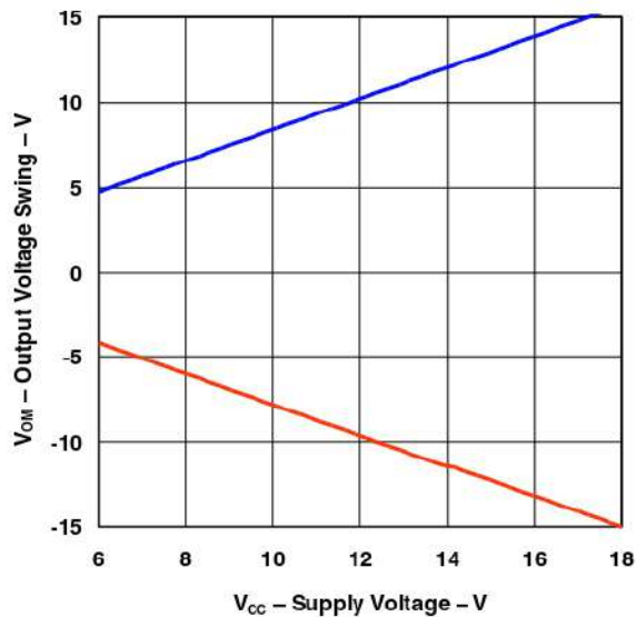
OUTPUT VOLTAGE SWING
