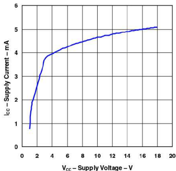
SUPPLY CURRENT vs SUPPLY VOLTAGE ( T_A = 25^\circ\text{C} )
