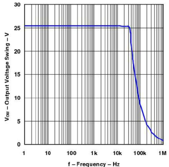
OUTPUT VOLTAGE SWING
