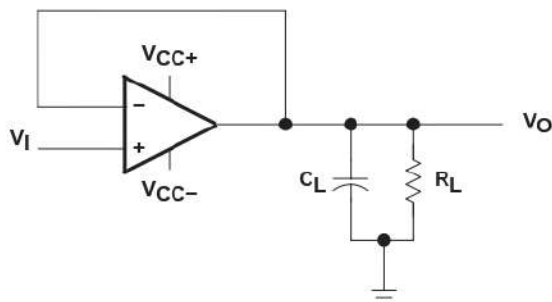
Figure 1. Unity-Gain Amplifier
