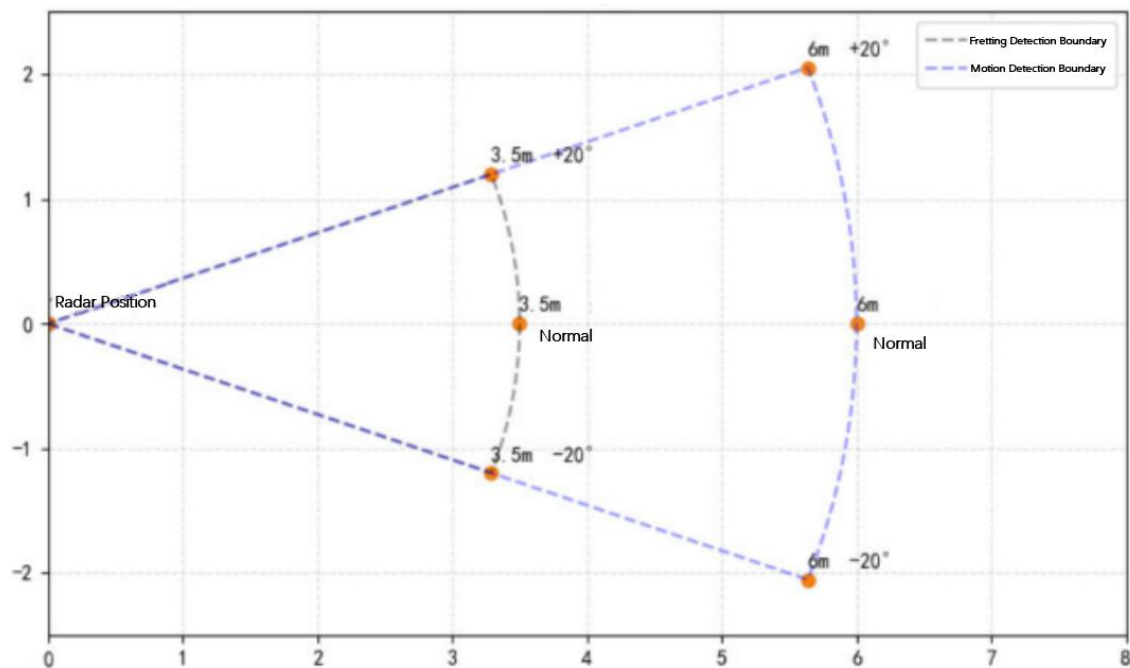
Figure 11 Power map of precision ranging wall-mounted radar
