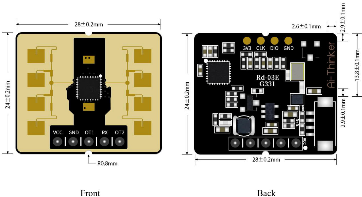
Figure 3 Appearance diagram (rendering diagram is for reference only, subject to the actual object)
