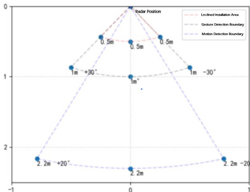
Figure 13 Schematic diagram of gesture recognition detection range
