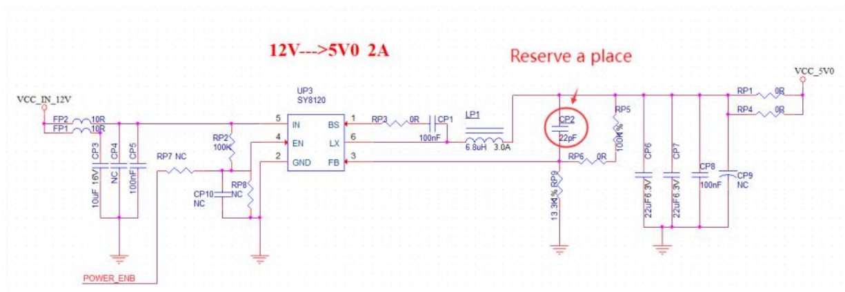
Figure 15 DC-DC step-down circuit diagram
