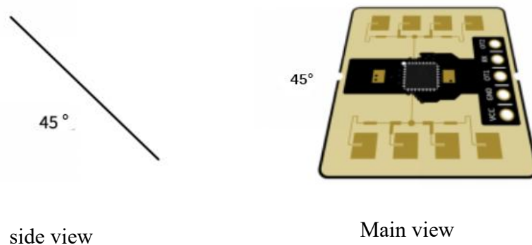
Figure 12 Schematic diagram of tilted installation for gesture recognition
