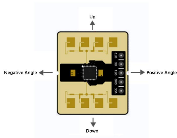
Figure 13 Schematic diagram of gesture recognition detection range
