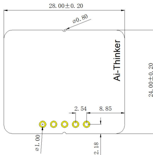
Figure 8 Recommended PCB package size
