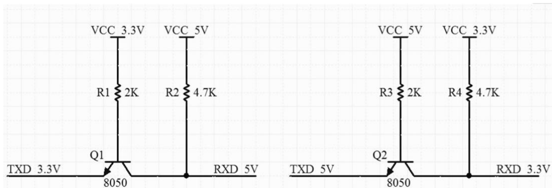
Figure 16 Level switching circuit
