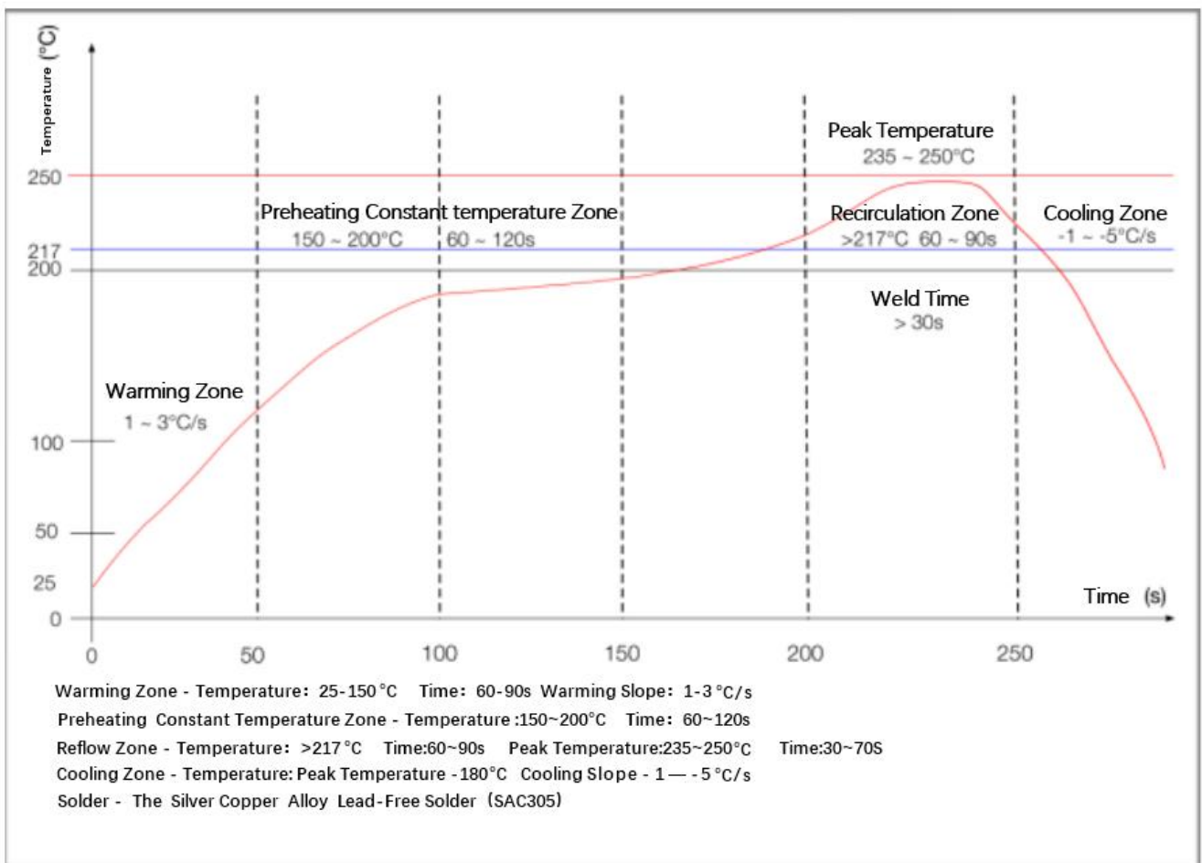
Figure 17 Reflow welding curve
