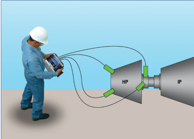
The AMS 2140 provides four-channels of simultaneous data collection plus phase, delivering real-time views into the most complex machinery problems.
