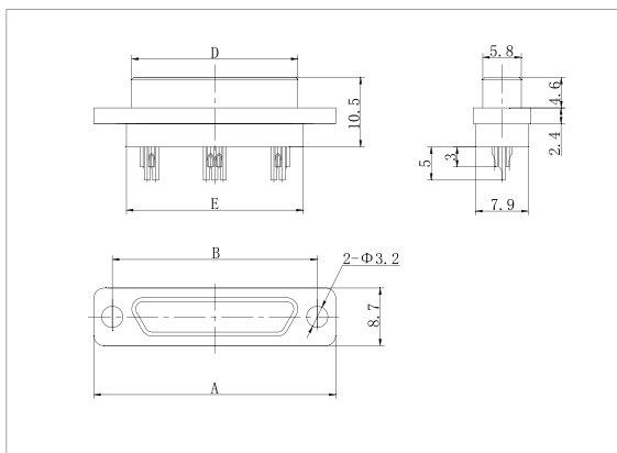
J30J-51~66TJS
