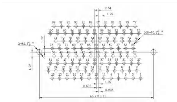
J30J-100TJN□
