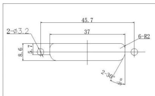
100 芯板后安装开孔尺寸
