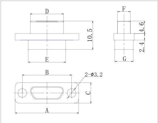
J30JR-□TK
