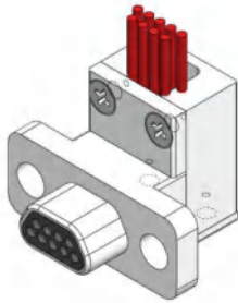
J30J-9TJ-C1
