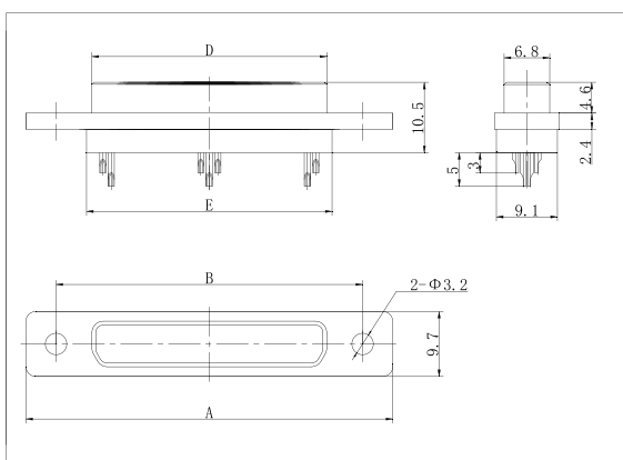
J30J-74~144TJS
