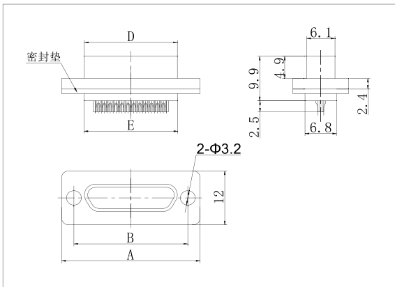
J30JM1-9~37ZKS
