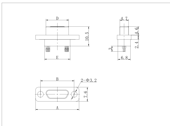
J30J-9~37TJS
