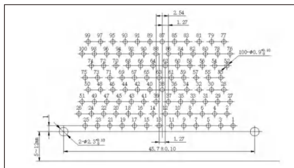
J30J-100TJW
